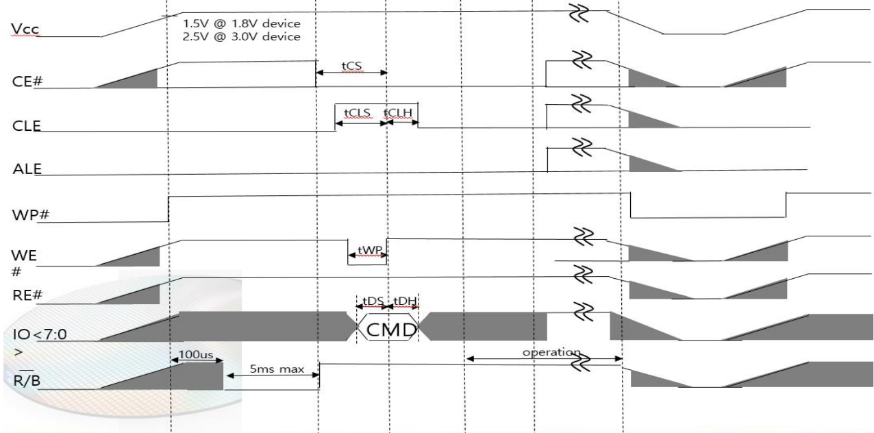
Figure 26 : Power up time sequence
