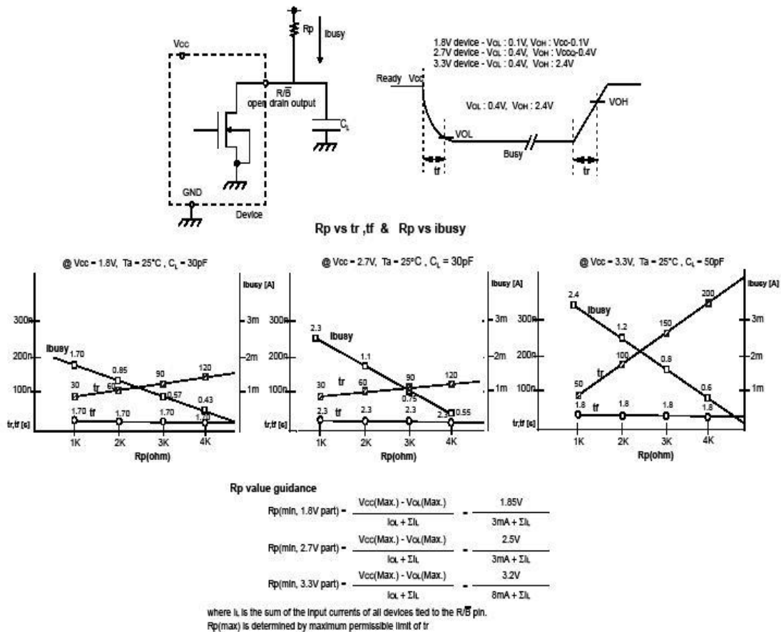
Figure 27 : Ready/Busy Pin electrical application
